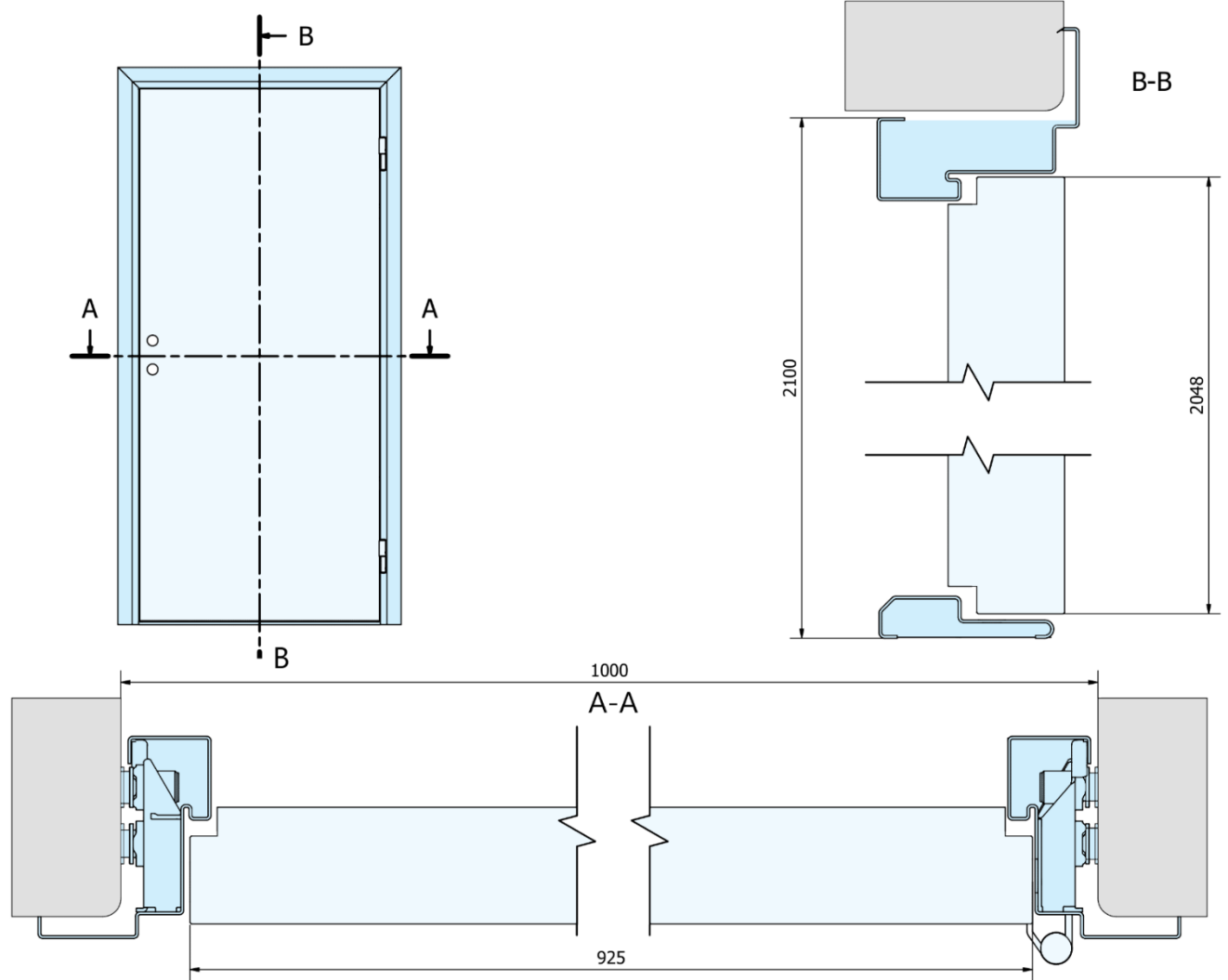
Figure A1: Wall and door dimensions
